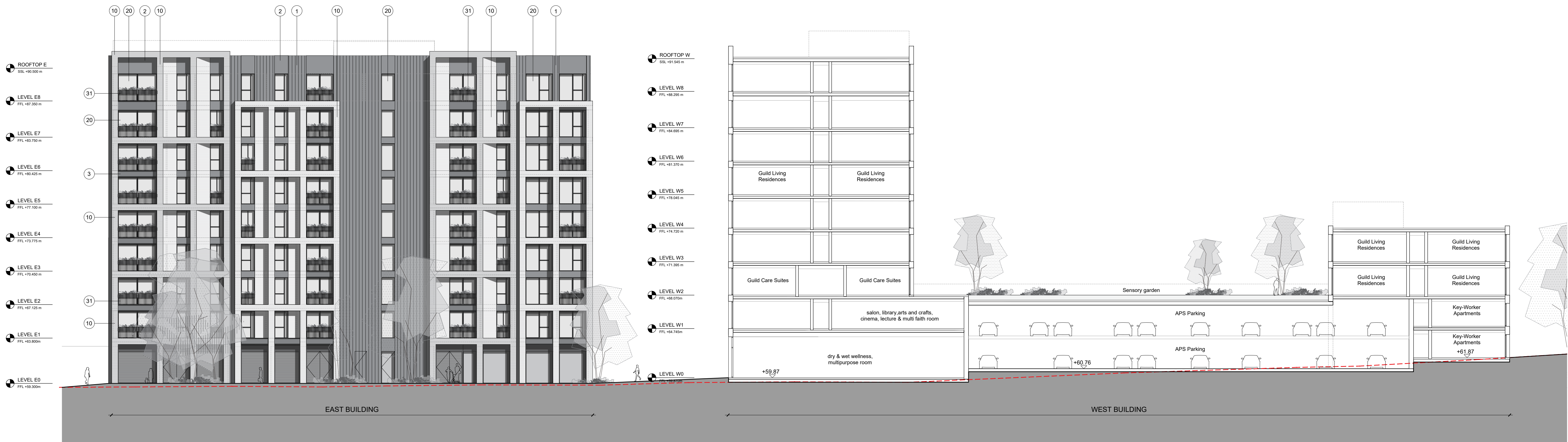
ELEVATION 11-11 1 : 200
