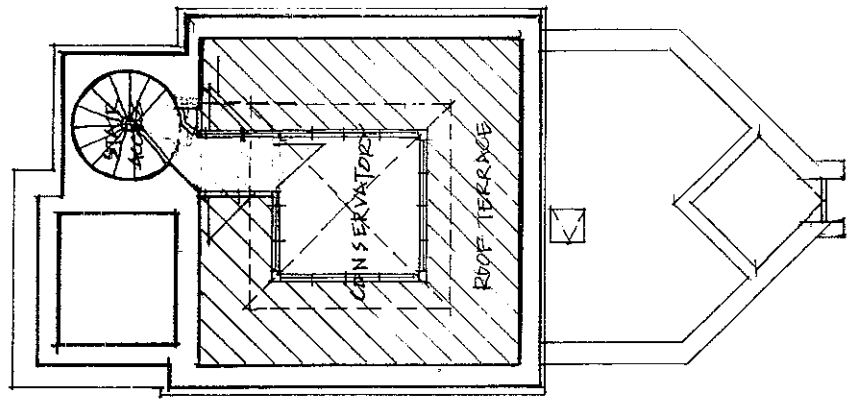
TWELFTH FLOOR TERRACE
