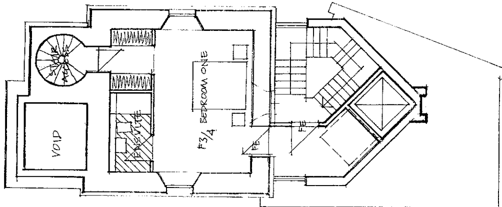
FIFTH FLOOR NINTH FLOOR SIMILAR
